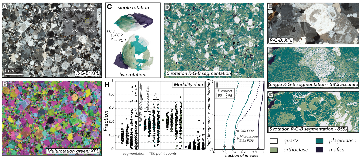
Figure 3. Improved modality data from multiple rotations of crossed polarizers for transmitted light imagery of thin sections. (A) Red-green-blue (RGB), cross-polarized (XPL) image of a granite thin section from the Golden Horn Batholith showing the full field of view (FOV) possible with our setup compared to those obtainable with a microscope camera. (B) False color image obtained using green (530 nm) light at three separate XPL orientations, 18° apart. (C) In principal component (PC) space, the pixel values for the four mineral classes (quartz, plagioclase, orthoclase, and mafics) in a single rotation RGB XPL image mostly overlap in one area of the plot. For an RGB XPL image containing five 18° rotations stacked into a 15-channel image, the pixel values spread out into a cone, where the position on the cone occupied by a given pixel relates to the class of the mineral and the relative orientation of its crystallographic axis. This added separation of the classes in the PC space of the five rotation XPL image improves the accuracy of pixel classifications from machine learning models, like the example given in (D). (E–G) In a zoomed-in portion of the image (E), we see that a support vector machine (SVM) using just a single rotation XPL RGB image (F) is 27% less accurate at classifying pixels compared to an SVM that is given the five-rotation image (G). Even with accurate classifications, analyzing only a relatively small FOV can add uncertainty. We see in (H) that the resulting modality data from the classification in (C) have highly variable values when assessed within the FOV of a traditional petrographic microscope. Each point in the plot represents the modality assessed in a randomly selected area of the segmentation equal to the size of a microscope FOV using either a 2.5× or 10× objective. The variation in these errors between classes stems from the characteristic size and relative abundance of the minerals. (I) To show the effect of crystal size and abundance, we calculate the number of images that correctly estimate the modality of a given mineral in a view size normalized to the mineral abundance (determined using a 4.5 × 5.5 × 4 cm 3D grinding, imaging, and reconstruction instrument [GIRI] reconstruction of the sample). In an experiment randomly drawing thin sections from the full volume of this granite sample, we see that an approximately equal fraction of images estimates the mafic mineral modality within a 90% correctness threshold when comparing GIRI to a 2.5× microscope objective. However, at the 95% threshold, as well as with the larger plagioclase crystals, the GIRI FOV performs nearly twice as well.
